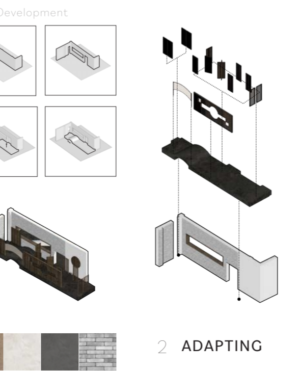
Kennedy's Sausage Factory and Shop Exploded Axonometric
