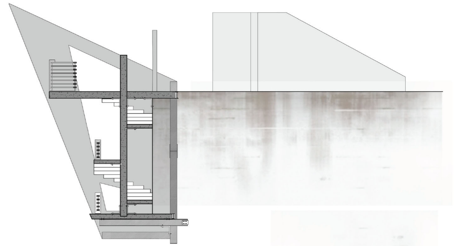
Long Section @ 1:200
