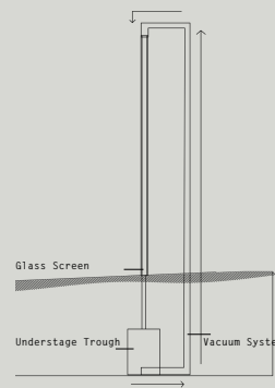
Sand Timer Structure Section
