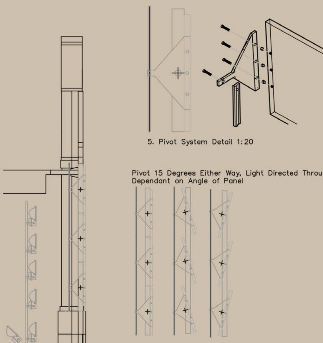
4. Pivot System Detail With Relevant Flood Lighting 1:50
