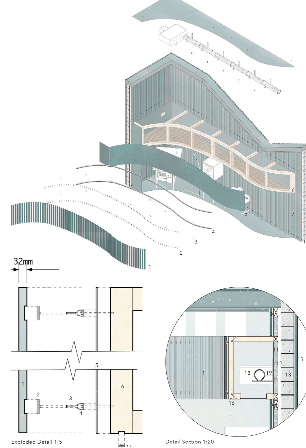
Exploded Detail 1:5
