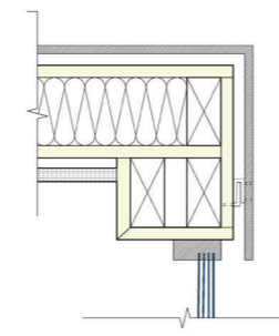
Detail B Ceiling to window joint.
