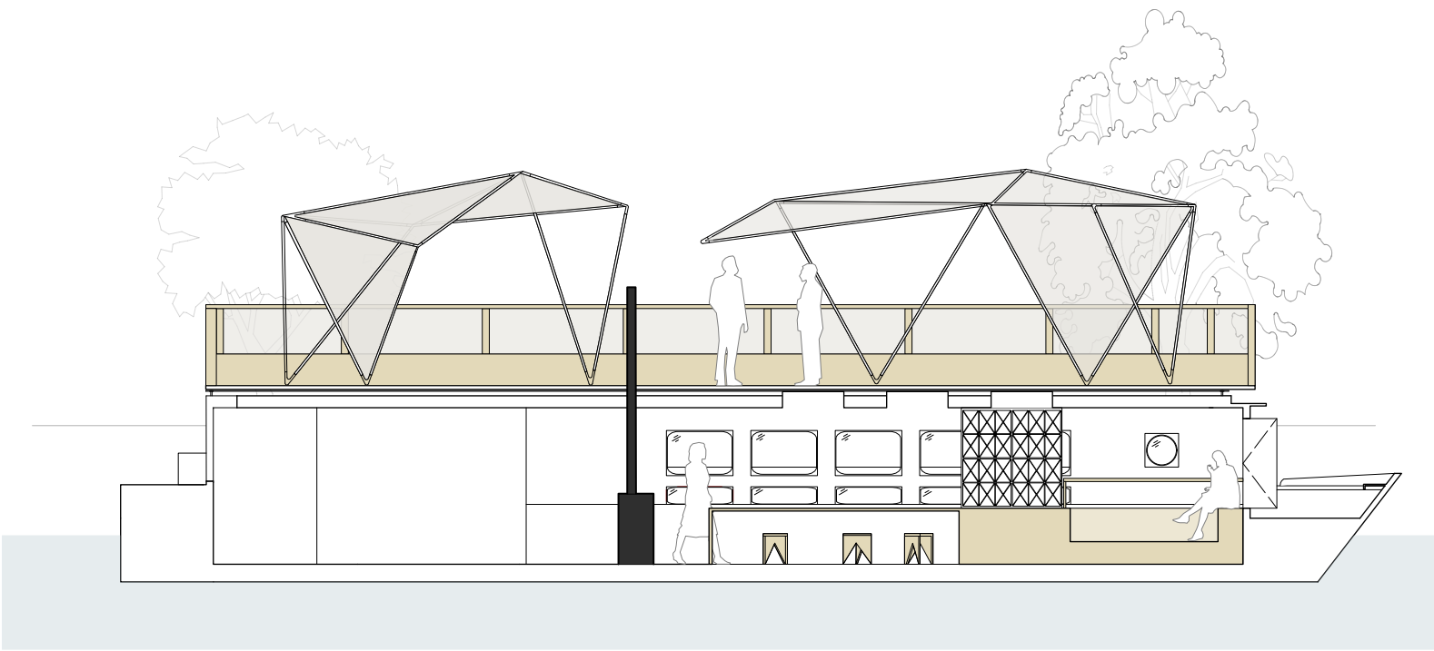
Section AA at 1:100
