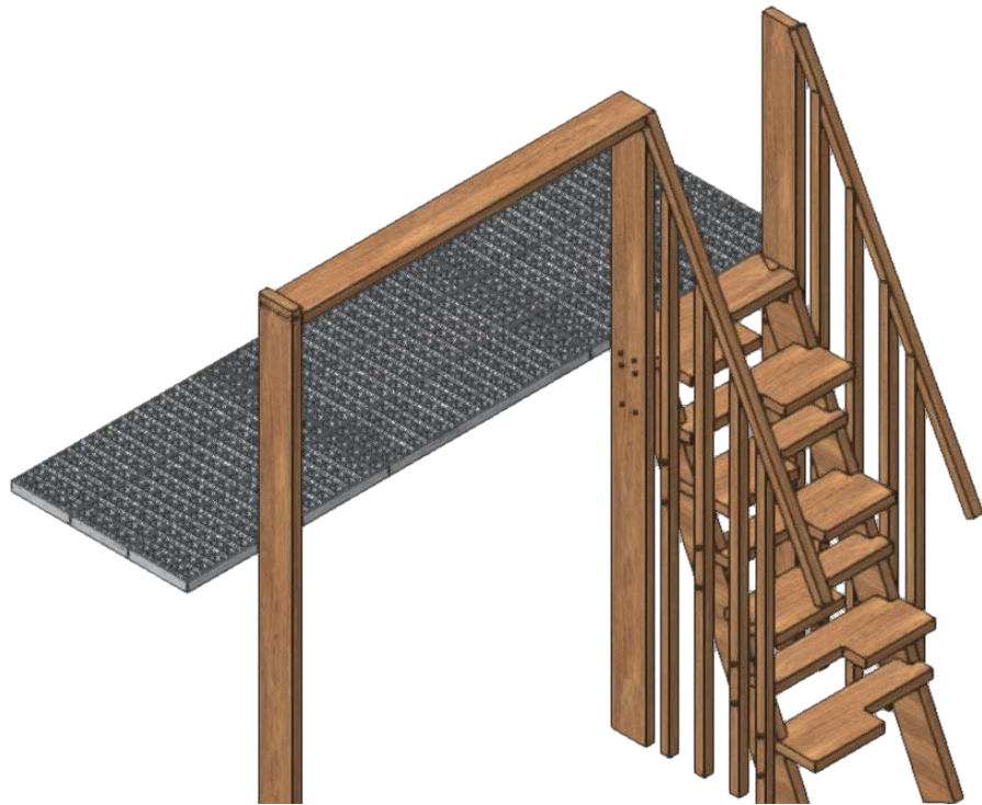
Platform Stairs Computer Model
