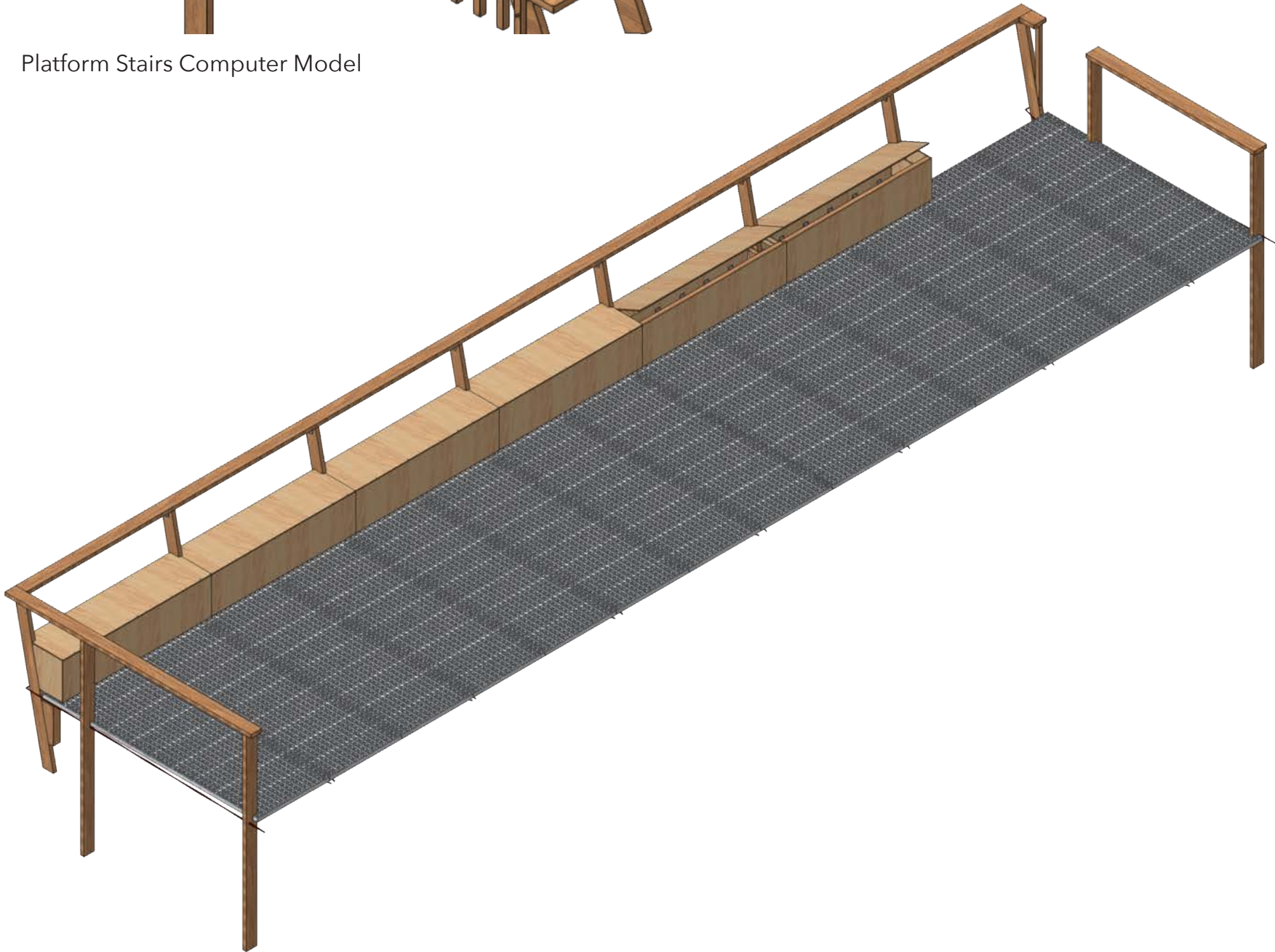
Platform Bench and Balustrade Computer Model
