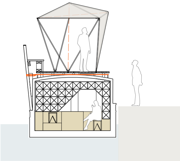
Section BB at 1:100
