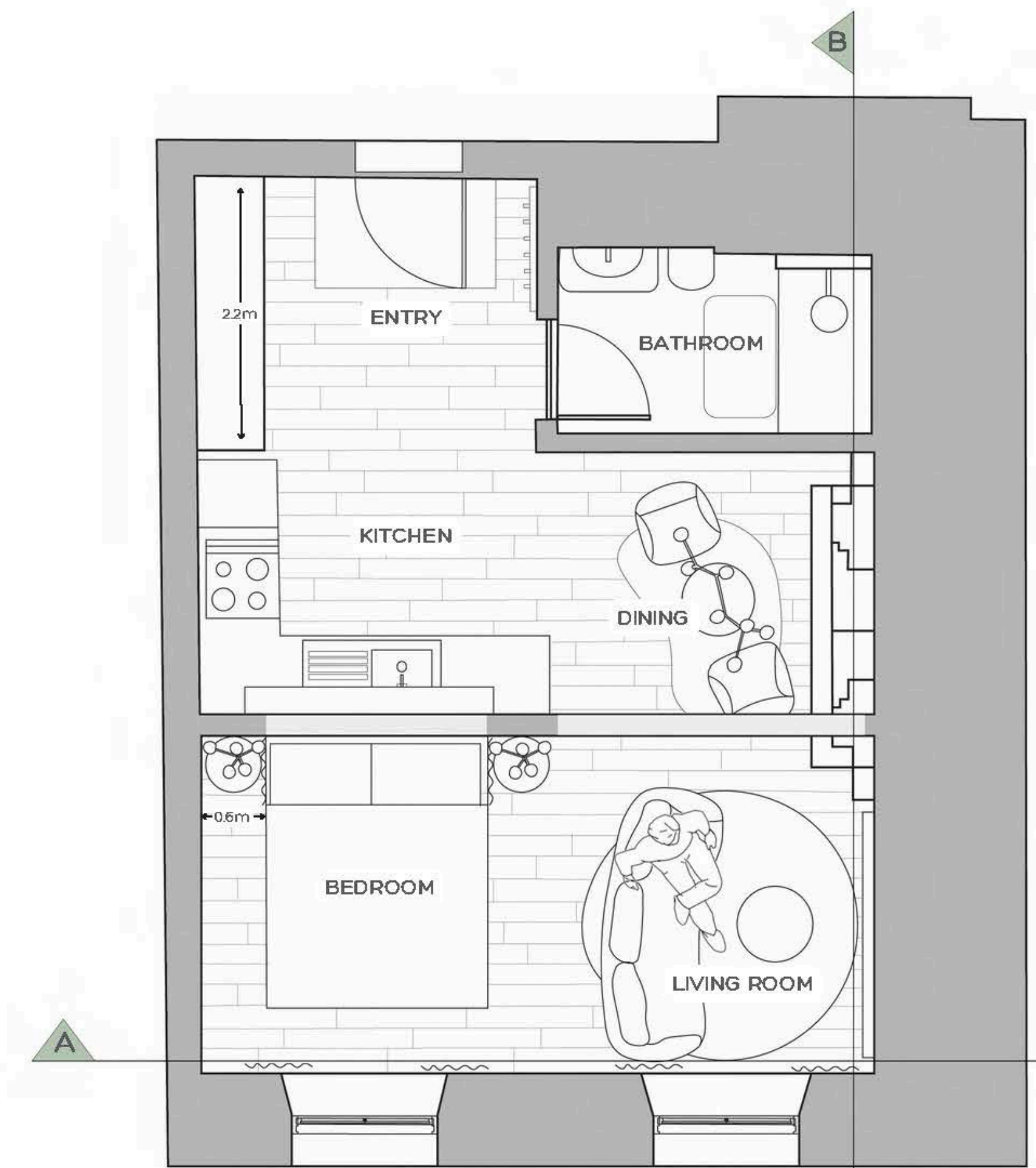
Plan drawing 1:50 @A3
