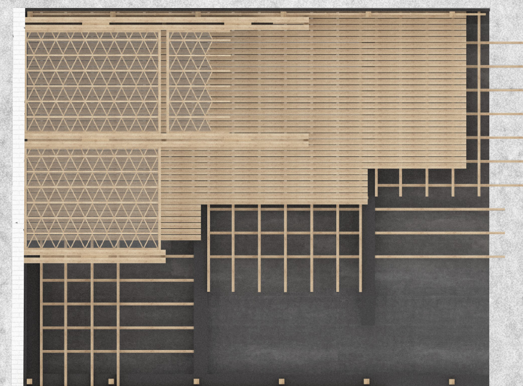
Roof construction detail plan
